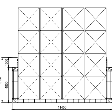
CROSS SECTION
